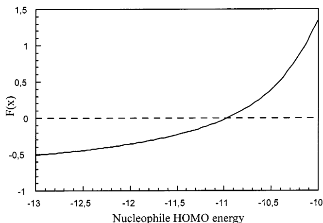
Figure 4. Plot of f(x) versus energy of the nucleophile HOMO
