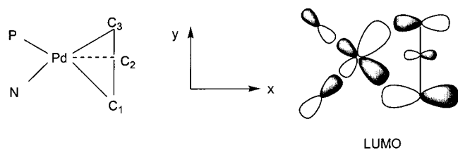
Figure 2. Projection of the model allyl-Pd complex on the xy plane and shape of its LUMO
