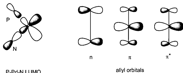
Figure 3. Shape of the LUMO of the P-Pd-N fragment and of the n , \pi and \pi^* orbitals of the allyl fragment
