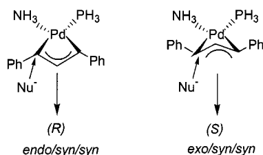
Figure 5. Most stable diastereoisomers of the model (\text{PH}_3)(\text{NH}_3) -(1,3-diphenylallyl)Pd complex
