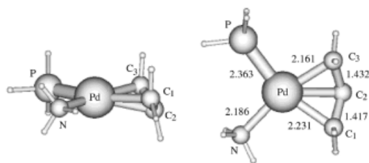
Figure 1. Optimized geometry for palladium complex Pd(NH 3 )-(PH 3 )( \eta^3 -allyl)
