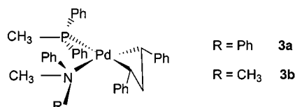
Figure 6. Modeling of the catalyst \text{Pd}(\text{CH}_3\text{PPh}_2)(\text{CH}_3\text{NPhR})(\eta^3\text{-1,3-diphenylallyl})
